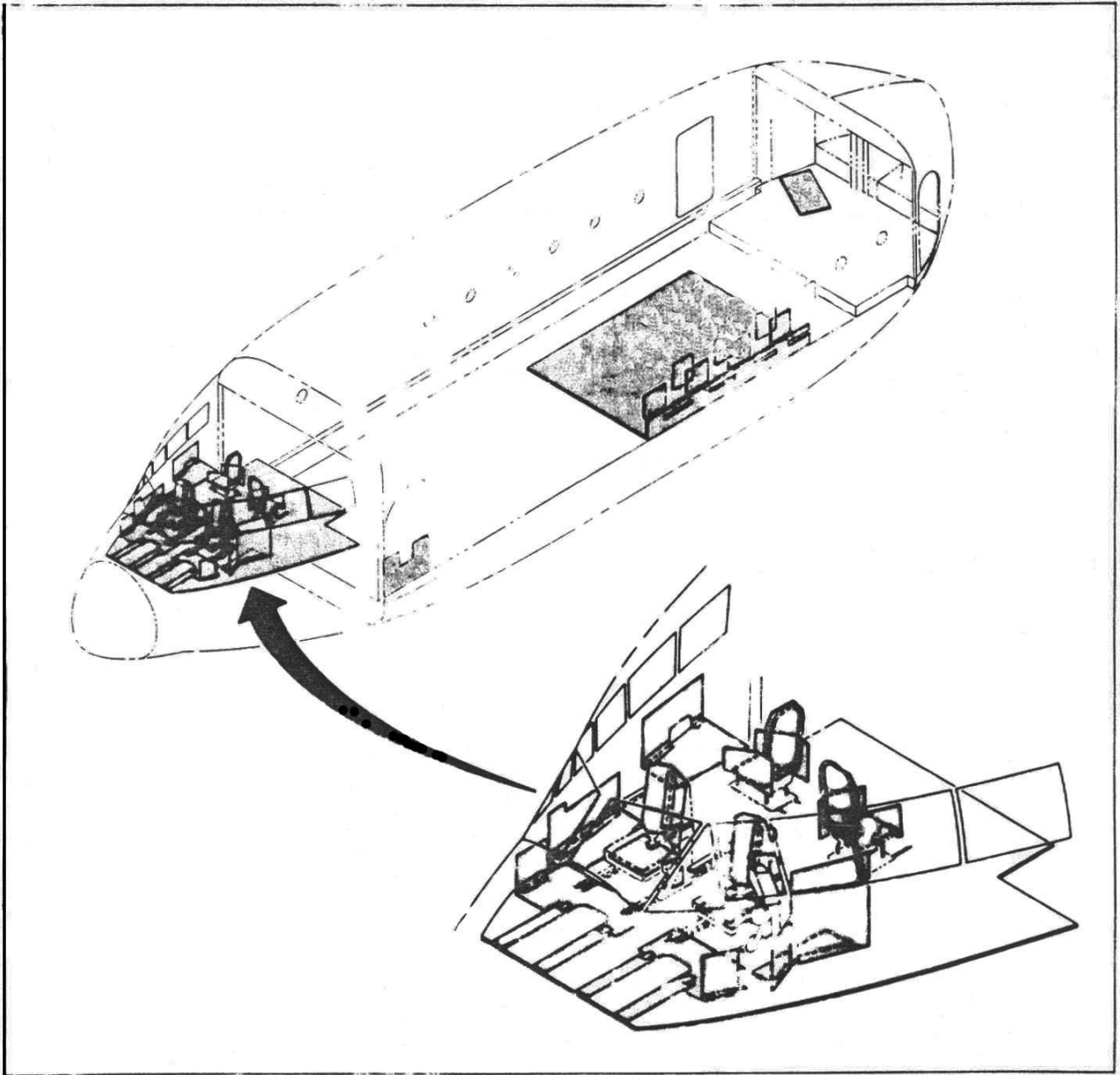
FIGURE 3-30. PROTECTIVE ARMOR PLATING
